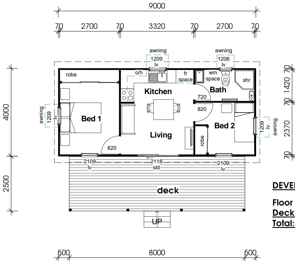
Floor Plan
