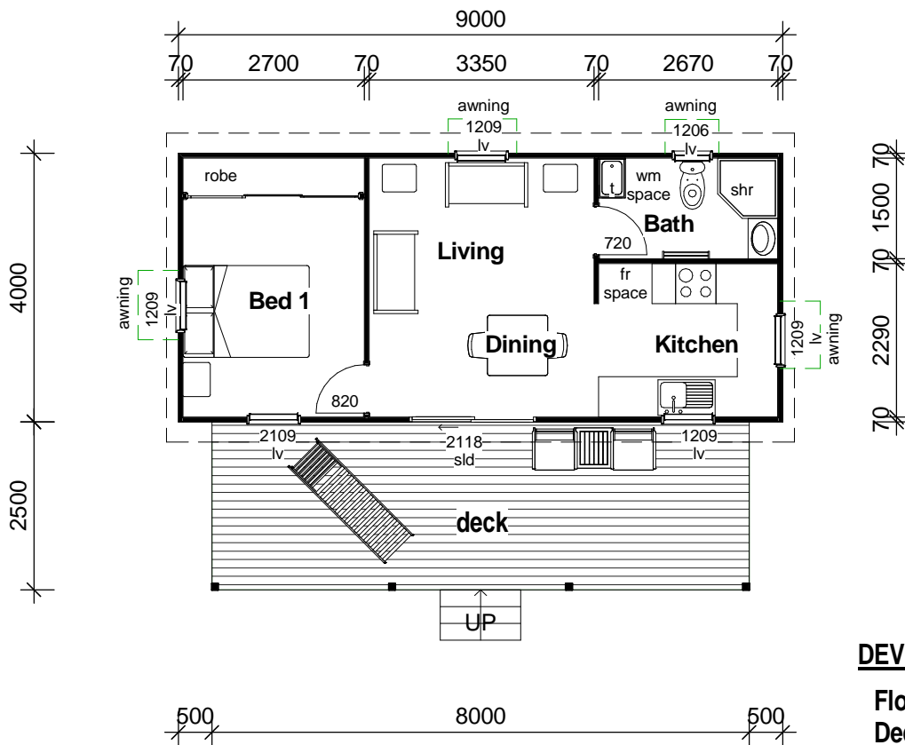
Floor Plan
